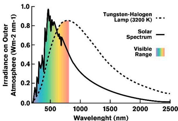
Figure S1. Irradiance spectrum of a Halogen lamp (3200K) compared to the solar irradiance on a surface per unit wavelength with emphasis on visible light range.
