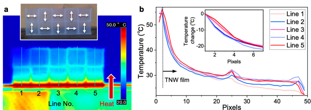
Figure 5. Thermal transport properties of the checked film of TNWs. (a) Thermograph of the film cantilevered by a hot-press machine at 60 °C. The insert shows a photograph of the cantilevered film with the patterning directions indicated by double-headed arrows. (b) Temperature profile on each line defined in (a) from the hot-press machine at the pixel of line 1. The insert shows the relative temperature change in each line from the holding end of the film.
