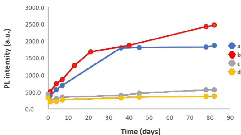
Figure 5. Influence of [\text{Cd}^{2+}]_{\text{F}}/[\text{thioacetamide}]_{\text{F}} at 4 °C. Temporal evolution of Photoluminescence intensity of CdS QDs solutions with different [\text{Cd}^{2+}]_{\text{F}}/[\text{thioacetamide}]_{\text{F}} ratios; (a) 4.0, (b) 2.0, (c) 0.8, (d) 0.4.
