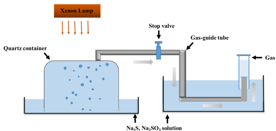
Figure S1. Schematic diagram of experimental arrangement for measurement.
