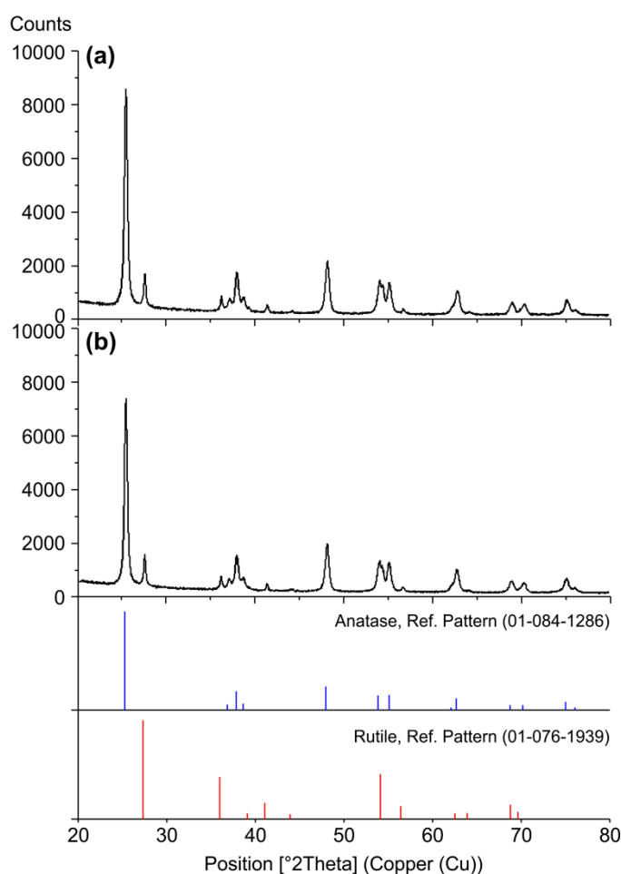
Figure S1. X-ray diffraction pattern (a) before and (b) after ultrasonic dispersion.
