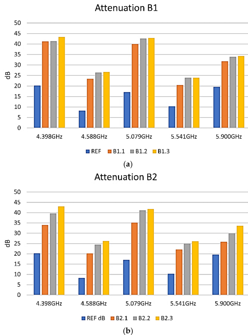
Figure 10. EMI-shielding measurements on B formulations samples. Blue reference, orange 1 layer, grey 2 layers, yellow 3 layers. (a) Graphic representation of EMI-shielding measurements results on B1 sample; (b) Graphic representation of EMI-shielding measurements results on B2 sample.
