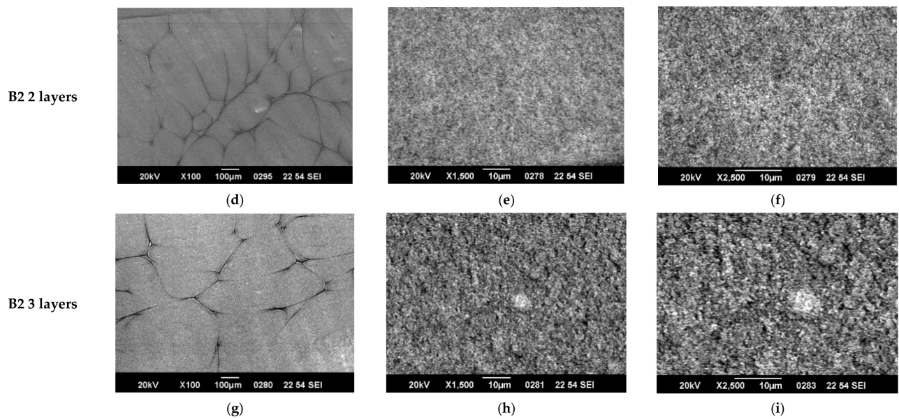
Figure 3. SEM characterization of 1, 2 and 3 layers of paint B2 at different magnifications. (a) B2.1 \times 100 (b) B2.1 \times 1500 (c) B2.1 \times 2500 (d) B2.2 \times 100 (e) B2.2 \times 1500 (f) B2.2 \times 2500 (g) B2.3 \times 100 (h) B2.3 \times 1500 (i) B2.3 \times 2500 .
