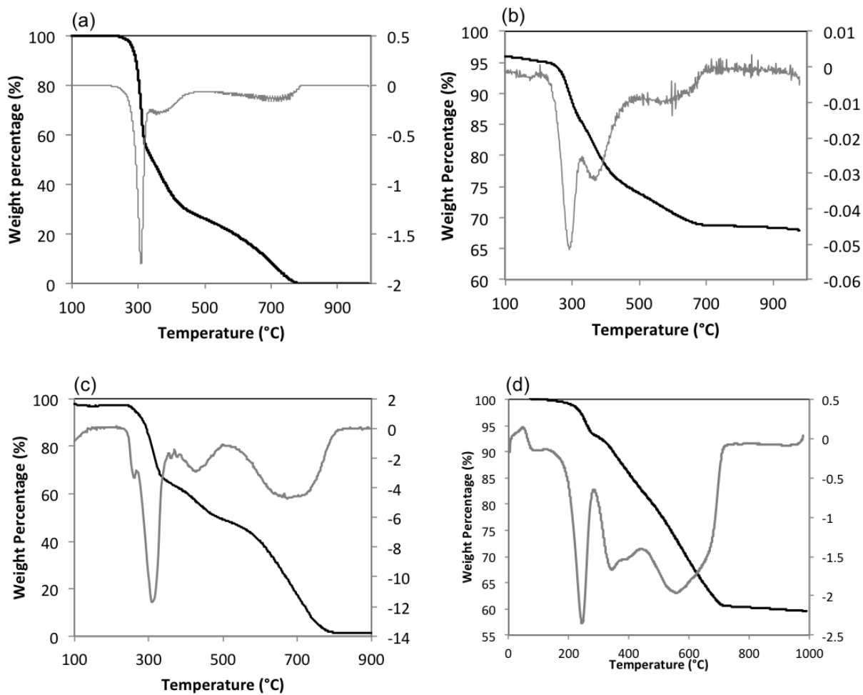
Figure S2. TGA curves of (a) PA-824; (b) AMS-6-PA824; (c) moxifloxacin; and (d) AMS-6-Moxi.
