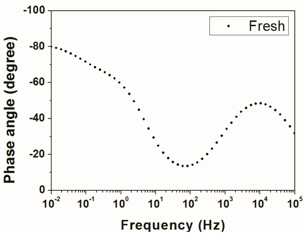
Figure S1. Bode plot of the fresh Co 3 O 4 nanorod electrode.
