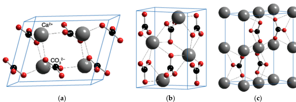
Figure 5. Crystal structures of the polymorphs of calcium carbonate. (a) Calcite; (b) Aragonite; (c) Vaterite.
