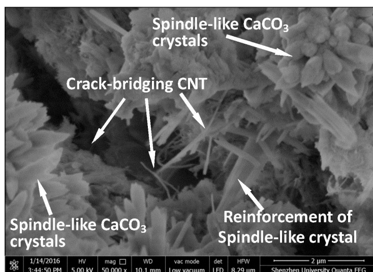
Figure 6. SEM image of C-CNT-CP broken sample.
