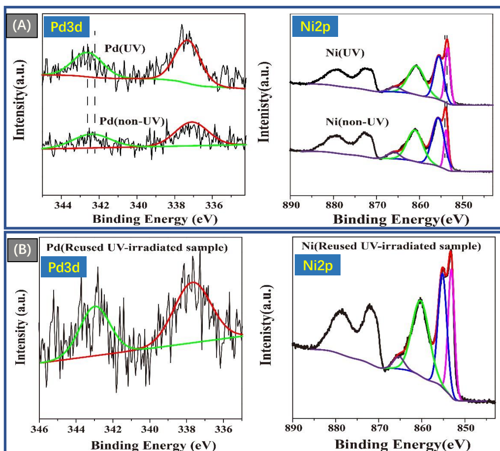
Figure 1S. XPS patterns of Pd and Ni elements of as-prepared Pd/NiO catalysts (A) and reused UV-irradiated Pd/NiO catalyst (B).
