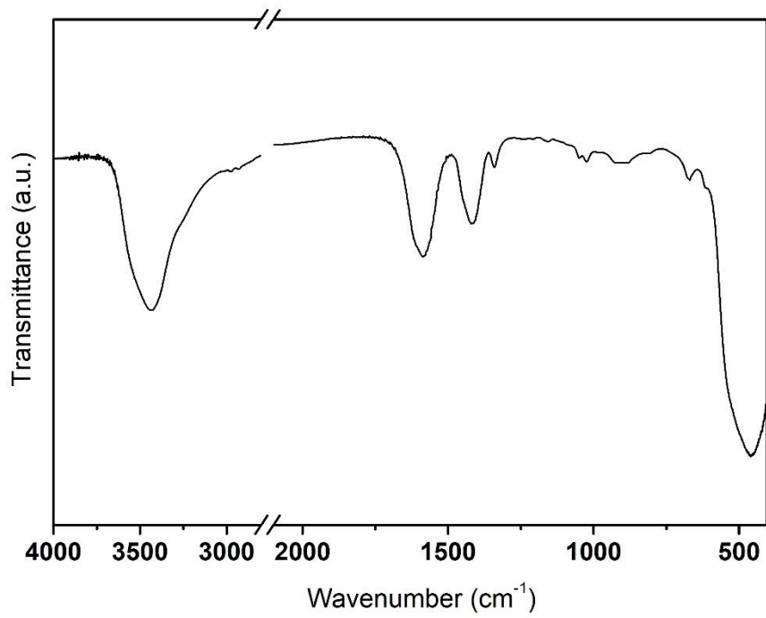
Figure S2. FTIR spectrum of \text{Co}_{0.15}\text{Zn}_{0.85}\text{O} .
