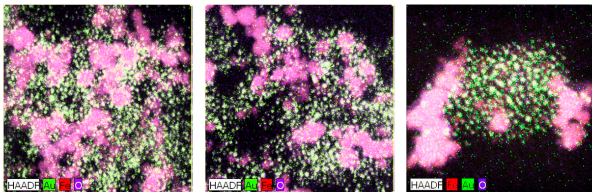
Figure S1: EDX elemental mapping-merged HAADF scanning TEM images of the type 1 NanoIOGs produced at 0.02 wt. % PEI.
