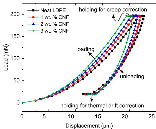
Figure S1. Representative load-displacement curve with no “nose” effect with holding time as 50 s.
