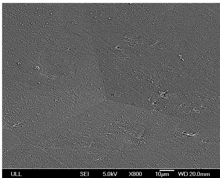
Figure S2. SEM image of a single indent in 2 wt. % CNF/LDPE showing no pile-up effect
