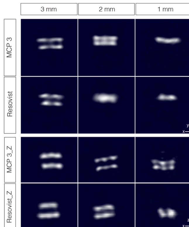
Figure 11. Dual-tube phantoms of 3, 2, and 1 mm inner diameter, filled with 1 mmol Fe/l MCP 3 and Resovist® and measured in two orientations. Images are interpolated and represented as maximum intensity projections with the threshold set at 50%.
