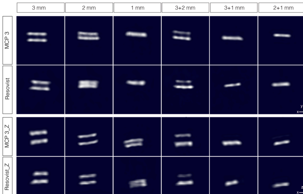
Figure 10. Dual-tube phantoms combining tubes of identical and different inner diameters (of 1, 2, and 3 mm) with MCP 3 and Resovist® at 10 mmol Fe/l and measured in two orientations. Images are interpolated and represented as maximum intensity projections with the threshold set at 50%.
