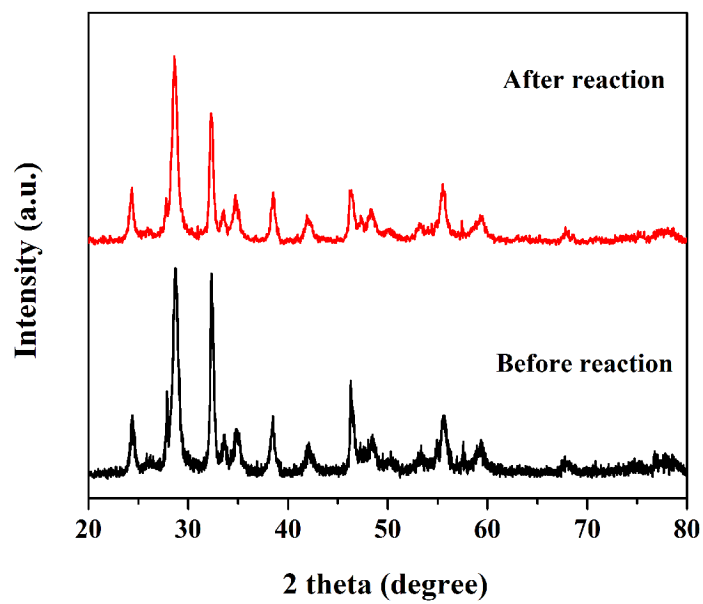
Figure S1 XRD patterns of the original and recovered Ag/AgCl/BOCH-3.
