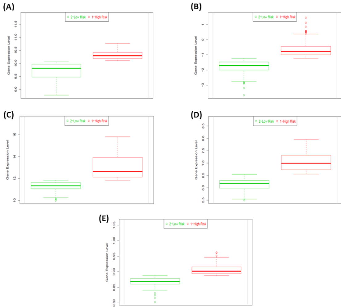
Figure S2. Box plot of TXRND1 mRNA expression across the two expression groups for (A) brain (GSE42669), (B) breast (TCGA-BRCA), (C) head & neck (TCGA-HNSC), (D) lung (GSE 30219) and (E) pancreas (PACA-AU) cancer datasets. P-values were calculated using t-test.
