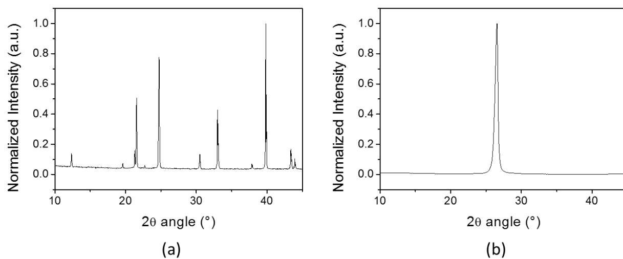
Figure S 1 Collected XRD diffractograms for (a) SrBr 2 ·6H 2 O and (b) Expanded Natural Graphite.
