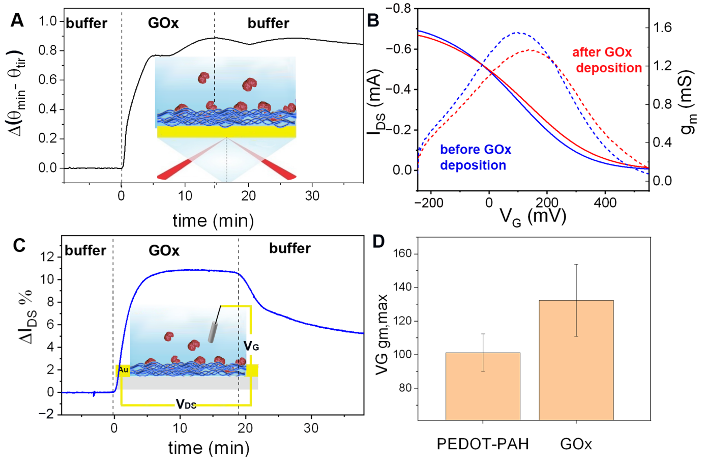
Figure 4. (A) Real time change in the SPR signal \Delta(\theta_{\min} - \theta_{\text{tir}}) during GOx deposition on a gold substrate modified with PEDOT-PAH under flow conditions. (B) Transfer curves and g_{\text{m}} vs. V_{\text{G}} of a PEDOT-PAH OECT in 10 mM KCl and 1 mM HEPES pH = 7.2 before (blue) and after (red) GOx deposition. (C) Relative change in the OECT I_{\text{DS}} current during GOx adsorption. (D) V_{\text{G gm,max}} changes (average of four devices. Error bars correspond to SD). V_{\text{DS}} = -50 mV and V_{\text{G}} = 54 mV.
