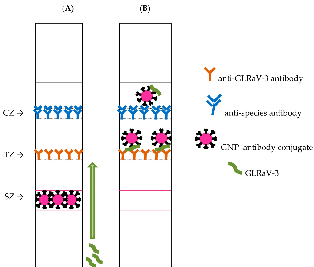
Figure 1. Scheme of the test strip for sandwich immunochromatographic assay (ICA) of GLRaV-3 before (A) and after (B) analysis.
