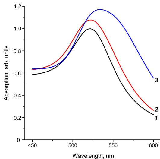
Figure 2. Absorption spectra of gold nanoparticles (GNPs). The mean sizes are 18.5 \pm 3.3 nm (1), 28.3 \pm 3.3 nm (2), and 51.0 \pm 7.9 nm (3).
