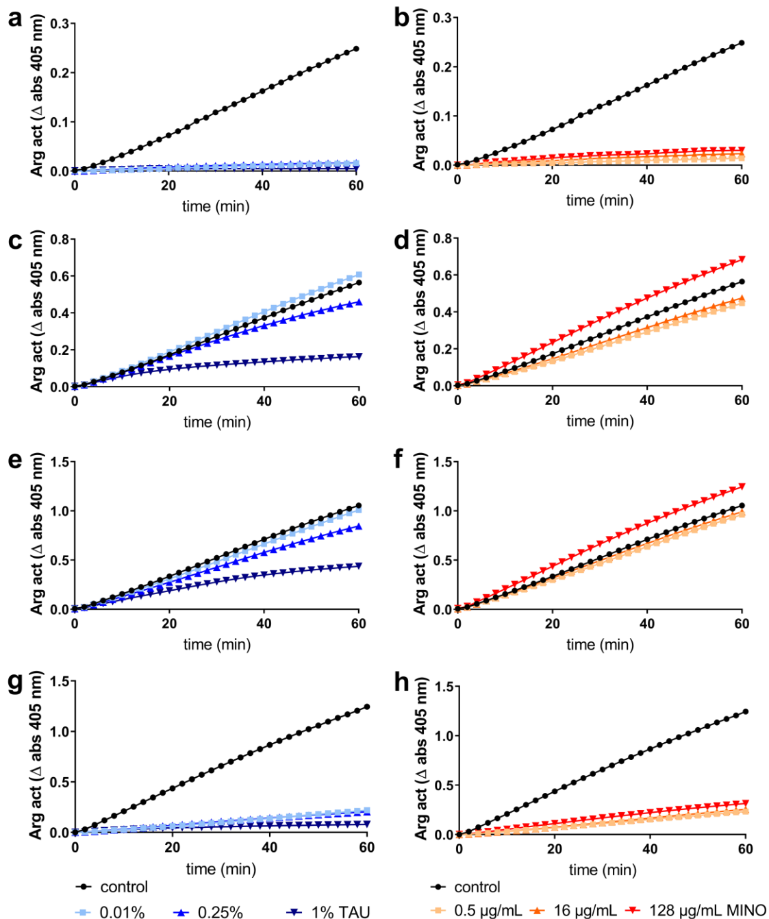
Figure 4. Arginine specific amidolytic activity (Arg act) measured by \Delta abs 405 nm after addition of taurolidine (TAU; a,c,e,g) and minocycline (MINO; b,d,f,h) in different concentrations to 10 nM RgpB (a,b), Porphyromonas gingivalis ATCC 33277 (c,d), P. gingivalis J374-1 (e,f) and P. gingivalis HG66 (g,h).
