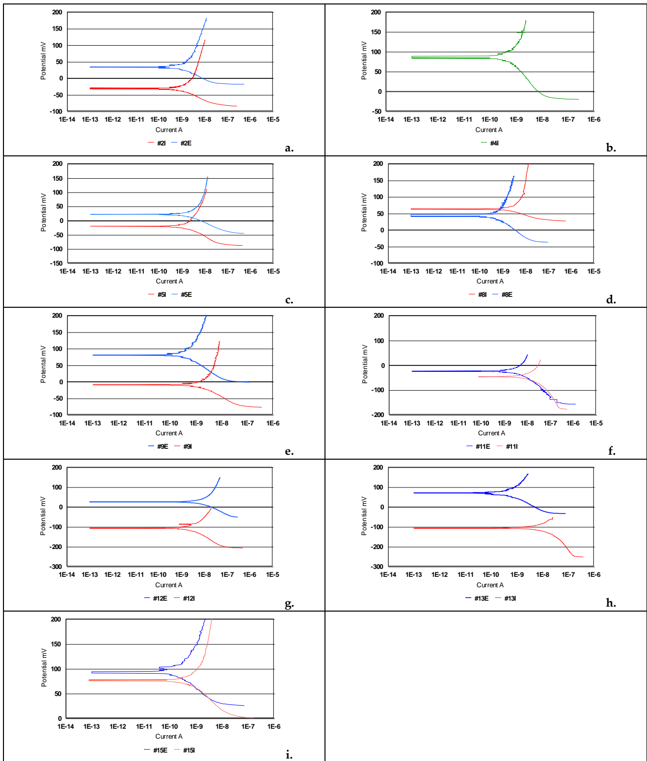
Figure S1. Polarization curves in the Tafel domain of the hypotubes: (a). #2(ref), (b). #4, (c). #5, (d). #8(ref), (e). #9, (f). #11, (g). #12, (h). #13(ref), (i). #15. E: external surface; I: internal surface.
