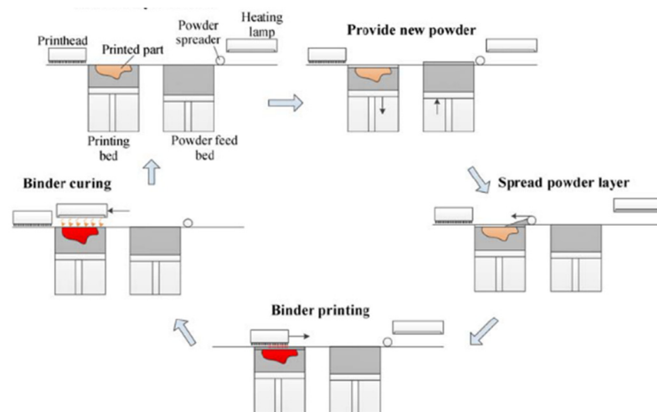
Figure 4. The schematics of BJ-AM process steps. Reproduced with permission from [86], Springer-Nature, 2018.
