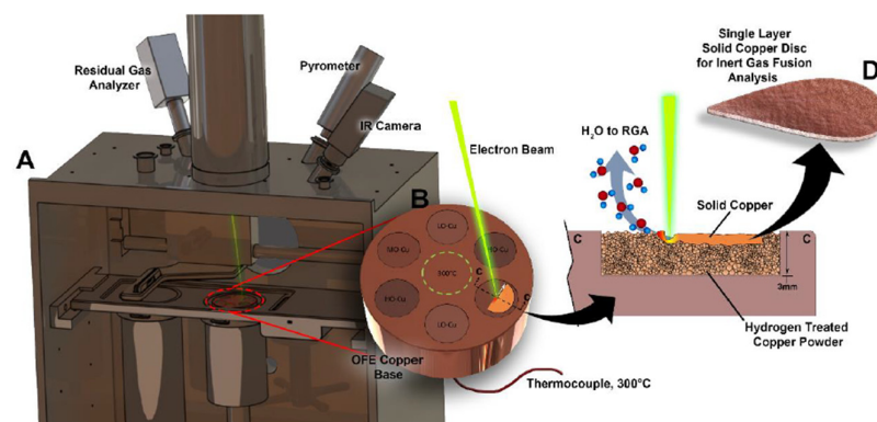
Figure 16. Description of in-situ H 2 O vapor outgassing experiment, (A) The diagram of the experimental instrument, (B) The base fixture contains six 3 mm deep pockets, (C) Powder melting process and detection, (D) The forming sample. Adapted from [6] MDPI, 2019.
