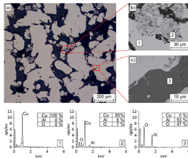
Figure 20. Microstructure of ODS-Cu processed via SEBM, (a) consists of three phases that are shown in (b,c). Reproduced with permission from [21] John Wiley and Sons, 2018.
