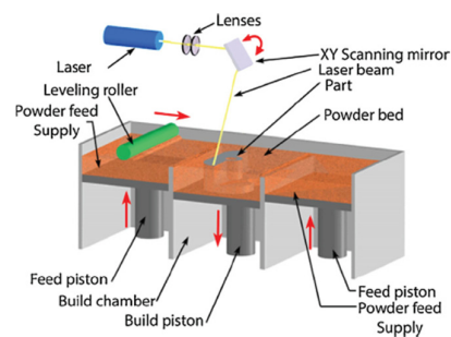
Figure 1. Schematics of additive manufacturing (AM) by selective laser melting (SLM). Reproduced with permission from [59], Elsevier, 2017.
