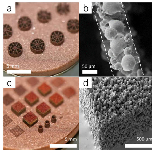
Figure 7. 3D image and SEM image of complex structures and block structure (a) 3D image of complex structures, (b) SEM image of complex structures, (c) 3D image of block structure, (d) SEM image of block structure. Reproduced with permission from [102], SpringerNature, 2017.
