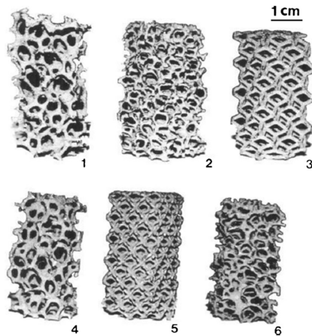
Figure 8. Examples of open cellular Cu mesh and foam specimens Stochastic foams are shown in (1), (2), (4) and (6); reticulated mesh samples are shown in (3) and (5). Reproduced with permission from [105] Elsevier, 2011.
