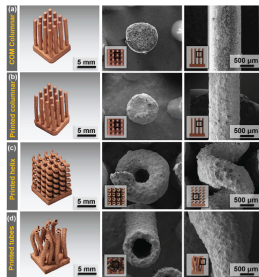
Figure 6. Top and side view photos (a) a commercial (COM) columnar, (b) a printed columnar, (c) a printed helix, and (d) a printed bent tubes heat sink. Reproduced with permission from [13], Elsevier, 2020.
