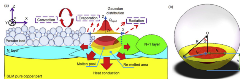
Figure 12. Schematics of heat transfer process of a molten pool during SLM processing (a) Heat transfer in laser molten pool during the SLM process; (b) simplified mathematical model of the laser molten pool. Reproduced with permission from [9] Elsevier, 2020.
