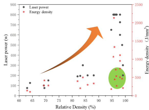
Figure 10. The relationship between laser power and relative density of pure copper part manufactured via SLM additive manufacturing [1,2,5,7,9,10,27,37,39–42,44].
