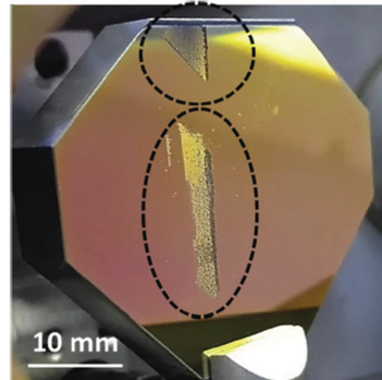
Figure 2. The damage to the optical mirror. Reproduced with permission from [39], Elsevier, 2019.
