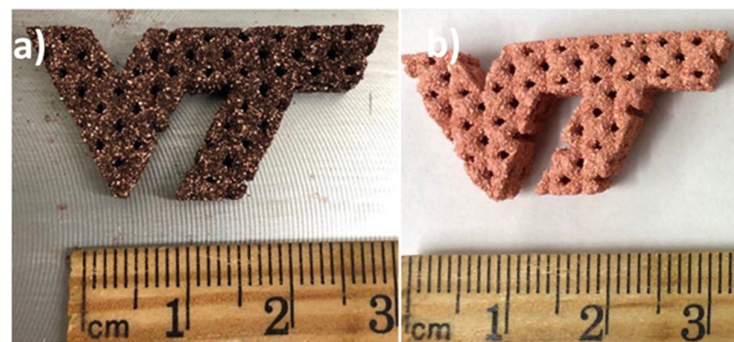
Figure 9. Copper foam part fabricated via AERO-Binder Jetting (a) green part (b) after sintering and annealing. Reproduced with permission from [99] Elsevier, 2020.
