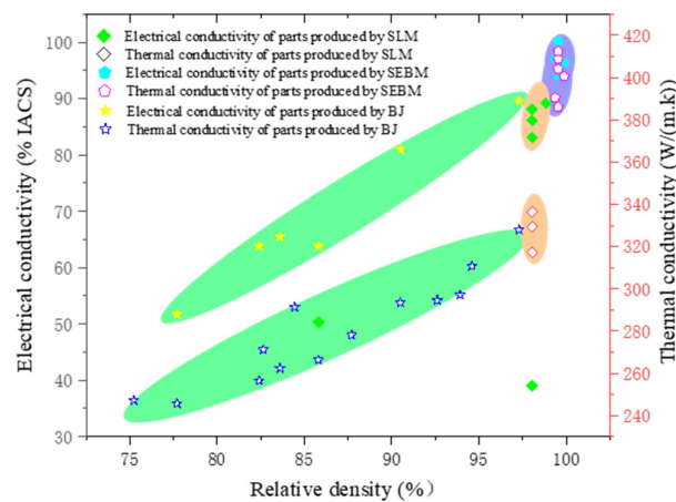
Figure 21. The relationship between electrical conductivity, thermal conductivity and relative density [1,4,7,27,38,39,47–49].
