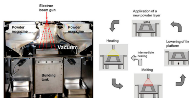
Figure 3. The SEBM process. Left: Process chamber. Right: 4-step process for building one layer. Adapted from [25], Maney Publishing, 2016.
