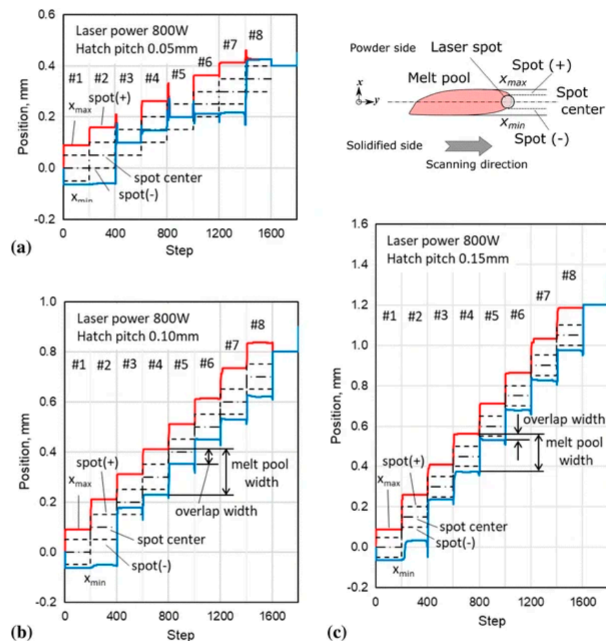
Figure 14. Positions of melt pool rim in x -direction (width) for hatch pitch of (a) 0.05 mm, (b) 0.10 mm, and (c) 0.15 mm. Reproduced with permission from [2] Springer Nature, 2017.
