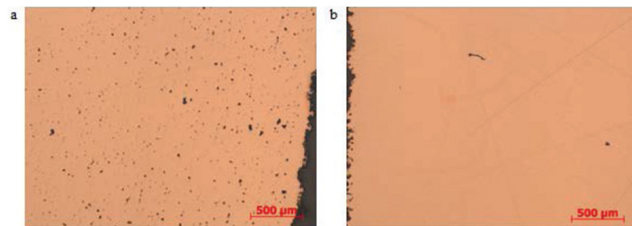
Figure 17. Sample micrographs indicating density improvement upon HIP, (a) Sintered Part, 1.88% porosity, (b) HIPed Part, 0.13% porosity calculated from image analysis. Adapted from [106] Elsevier, 2017.
