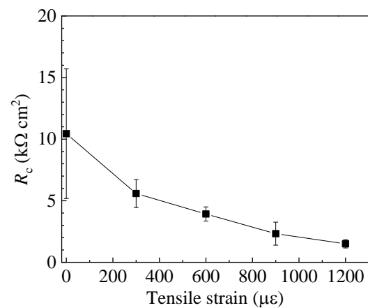
Figure 9. Effect of the tensile strain level on the enamel coating resistance.
