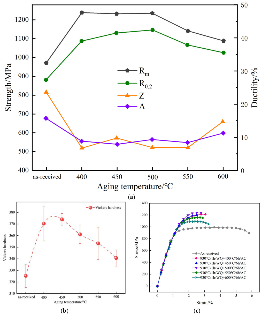
Figure 1. Effect of aging treatment on mechanical properties of Ti-5Al-3V-1.5Mo-2Zr titanium alloy drill pipe: (a) tensile property curve, (b) hardness change, (c) stress–strain curve (adapted from [21]).
