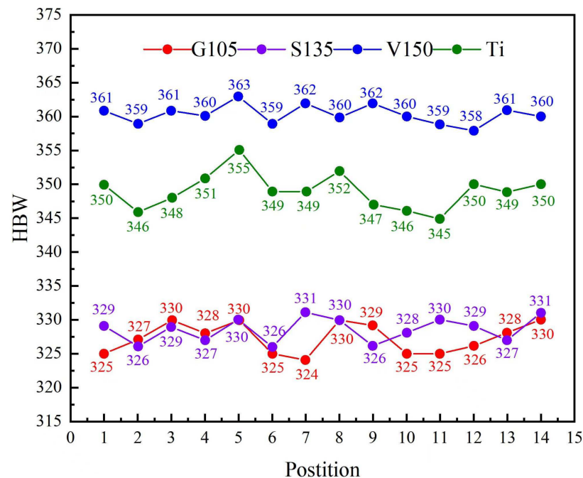
Figure 2. Hardness distribution of different drill pipes (adapted from [37]).
