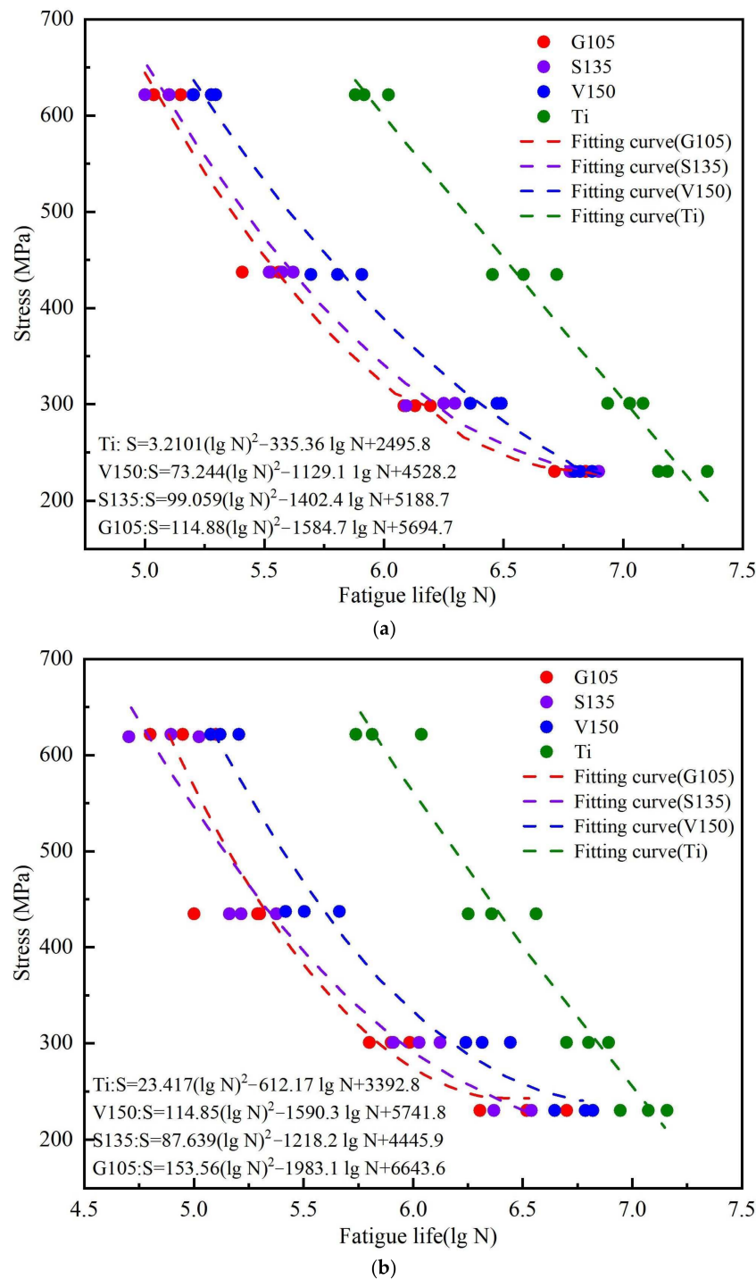
Figure 3. Fatigue curves of different drill pipe samples in H 2 S mud (a) at room temperature and (b) at 100 °C (adapted from [37]).
