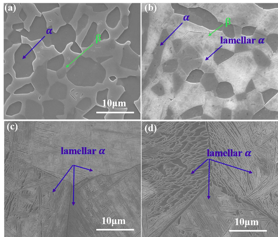
Figure 4. Microstructure of Ti-3Mo titanium alloys after annealing at different temperatures: (a) 750 °C, (b) 850 °C, (c) 950 °C, and (d) 1050 °C (adapted from [47]).
