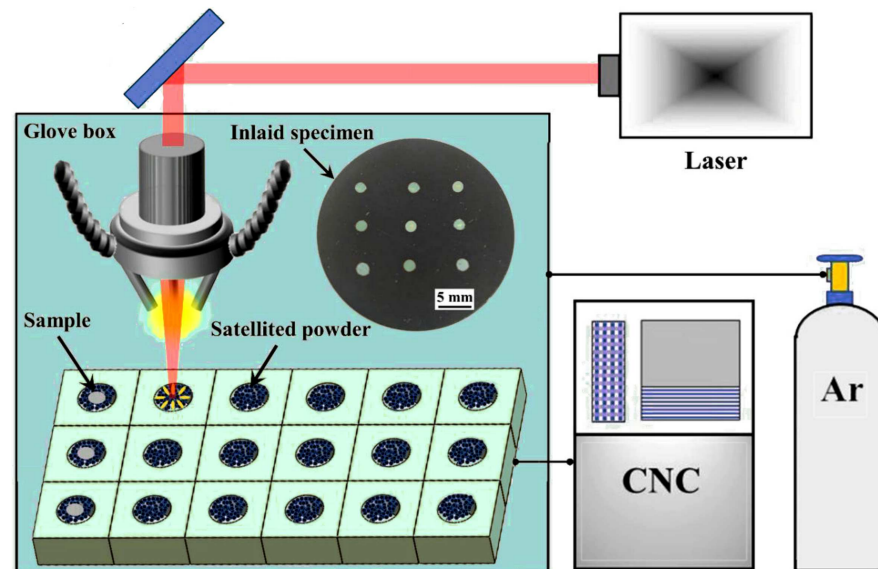
Figure 5. Schematic of the laser micro-alloying process and the inlaid specimen (adapted from [24]).
