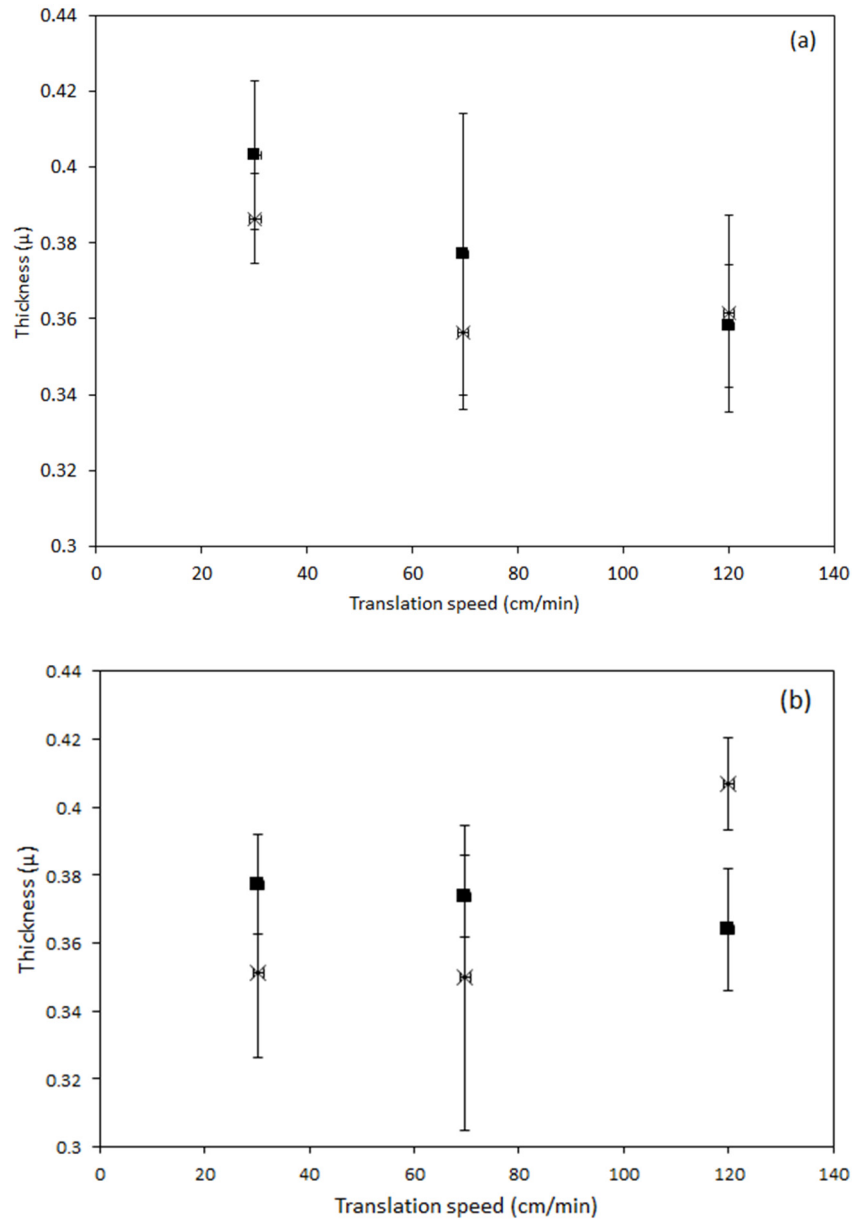
Figure S1. Film thicknesses at different translation speeds for ( \times ) 0.6M and ( \blacksquare ) 0.2M TFAA solutions using Sn/H 2 O ratio of (a) 1:5 and (b) 1:30.
