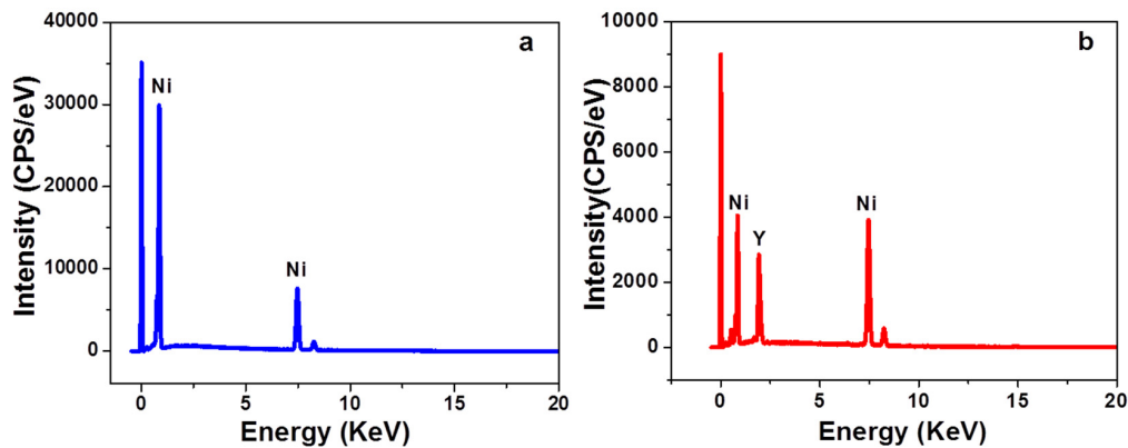
Figure 2. EDX analysis of electrodeposited Ni-B (a) and Ni-B- Y_2O_3 (b) composite coatings.
