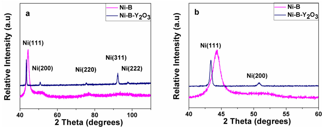
Figure 1. The large (a), and small scale (b) XRD spectra of electrodeposited Ni-B and Ni-B-Y 2 O 3 composite coatings.
