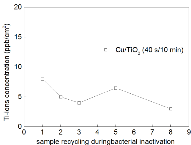
Figure 5. Ti-ions release from a diverse TiO 2 /Cu (10 min/40 s) cotton sputtered sample as a function of catalyst cycling up to the eighth cycle.
