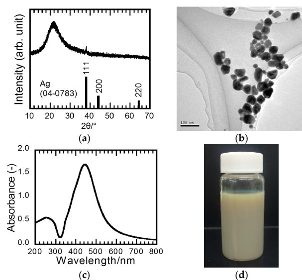
Figure 2. Silver colloid nanoparticles. (a) XRD pattern; (b) TEM image; (c) optical absorption spectrum; (d) optical image.
