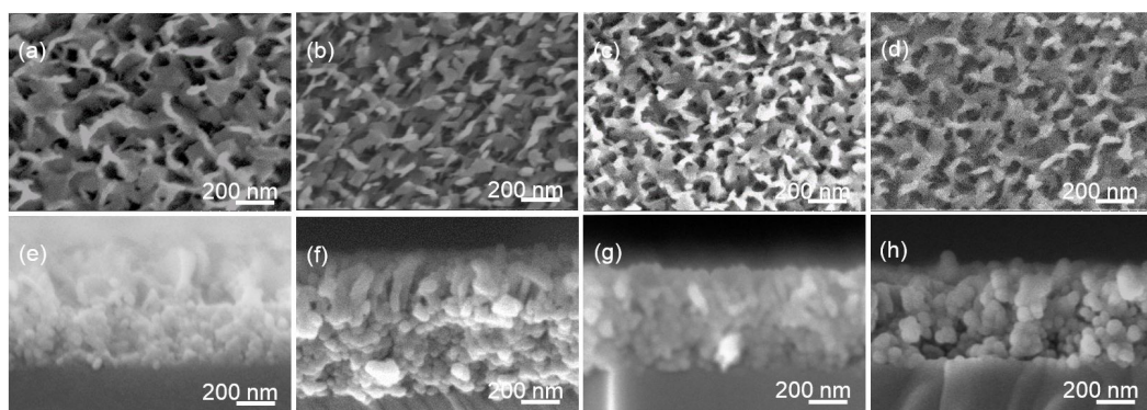
Figure 5. Surface (top) and cross-section (bottom) FESEM image. (a,e) Film-A2; (b,f) Film-B2; (c,g) Film-C2; (d,h) Film-D2.
