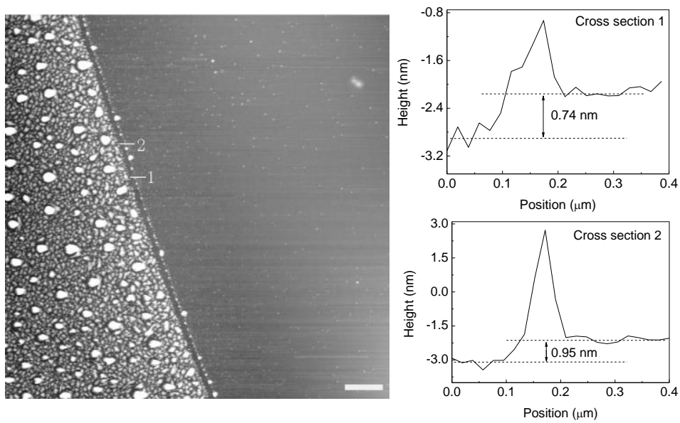
Figure S2. AFM image of monolayer MoS 2 showing the edge of the domain. Scale bar represents 1 \mu\text{m} in AFM image.
