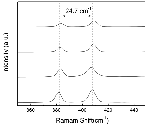
Figure S1. Raman spectra of a multi-layers MoS 2 growth on the SiO 2 /Si substrate tested at different locations, corresponding to the data in Figure 3a–d.
