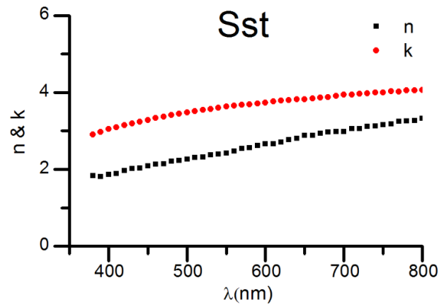
Figure S1. Complex refractive indexes of Sst.
