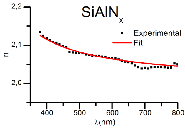
Figure S2. Refractive indexes of SiAlN x .
