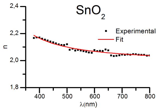
Figure S3. Refractive indexes of SnO 2 .
