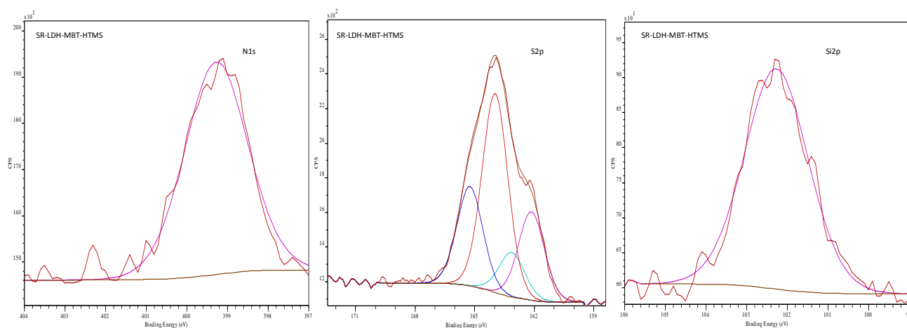
Figure S1. XPS spectra of SR-LDH-MBT after functionalization with HTMS.
