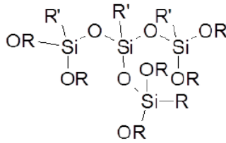
T 3 structure
