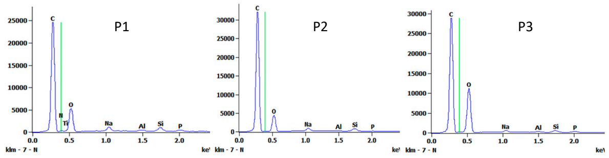
EDX analyses performed on the surface of the treated flax fibers
