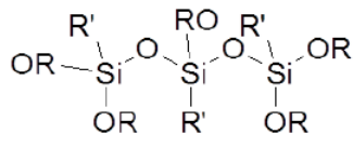
T 2 structure
