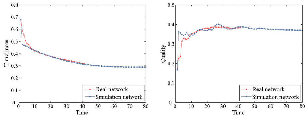
Figure 11. Simulation and empirical results of network timeliness and quality evolution.
