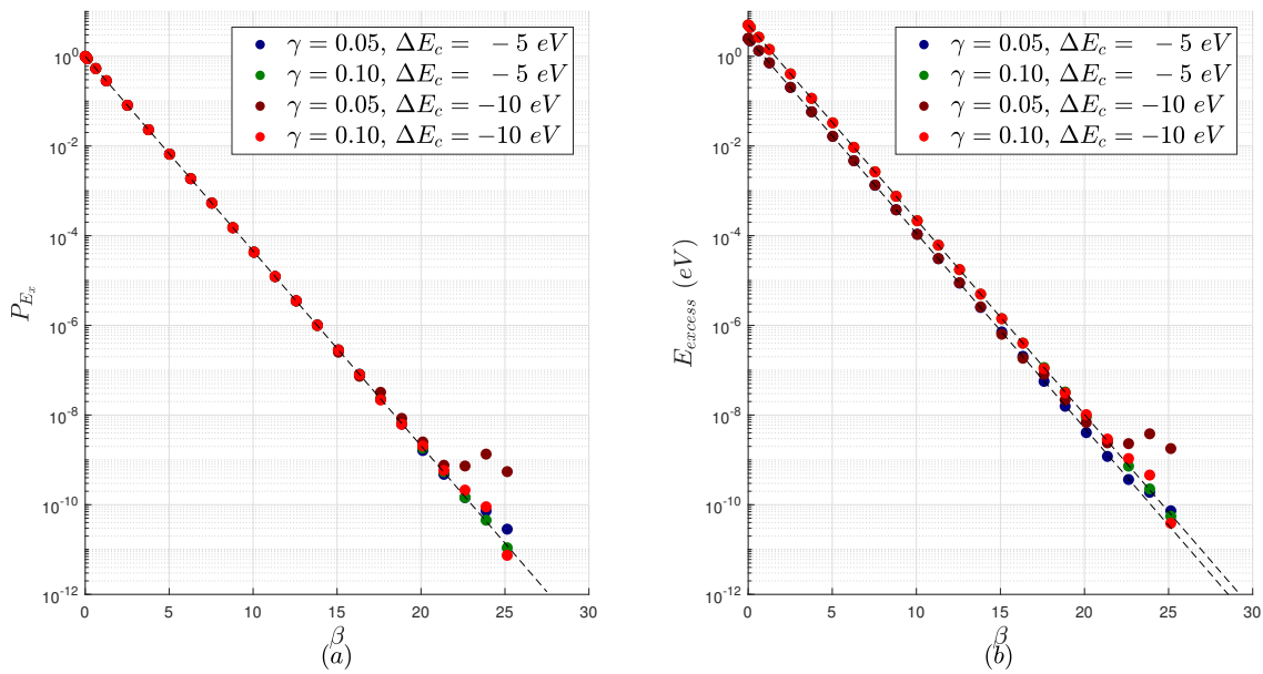
Figure 11. Adiabaticity of the ERASE WITH COPY operation. The use of a copy allows an erasure protocol in which the system is first biased so that the initial state is the ground state of the system, as shown in Figure 7b for a stored 1 bit. (a) Probability of excited state occupation ( P_{E_x} ) decreases exponentially with increasing adiabaticity. The dotted line represents the relation P_{E_x} = e^{-\beta} (Equation (17)). Deviation from the dotted line is at the tolerance level ( 10^{-9} ) of the numerical method. (b) Excess energy ( E_{excess} ) also decreases exponentially with increasing adiabaticity. The dotted lines represent the relation E_{excess} = -E_{c,final}e^{-\beta} (Equation (19)). P_{E_x} and E_{excess} depend on the value of \beta and not on individual values of \gamma , \Delta E_c and T .
