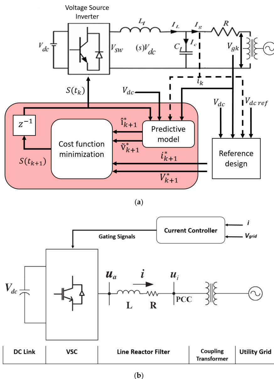
Figure 6. (a) Single-phase MG system, (b) the test system with one-line diagram.
