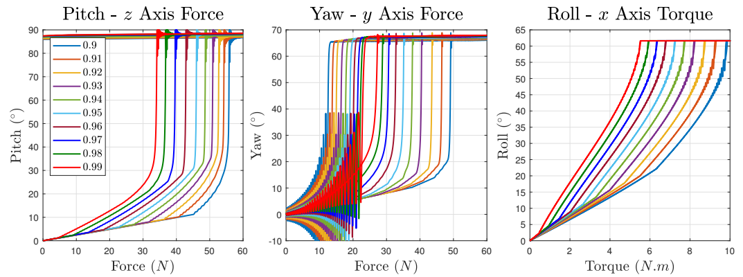
Figure 4. The rotation caused by the force or torque applied on the free-moving module. (Left): The pitch motion caused by applying the force along the z axis of the free-moving module. (Middle): The yaw motion caused by applying the force along the y axis of the free-moving module. (Right): The roll motion caused by applying the torque along the x axis of the free-moving module.
