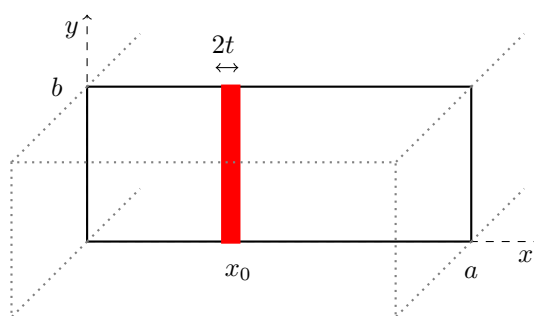
Figure 1. Geometry of the problem; thin strip of width 2t inside the rectangular waveguide.
