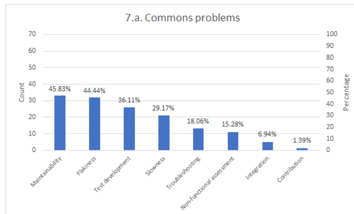
Figure 16. Categories for common problems related to Selenium.
