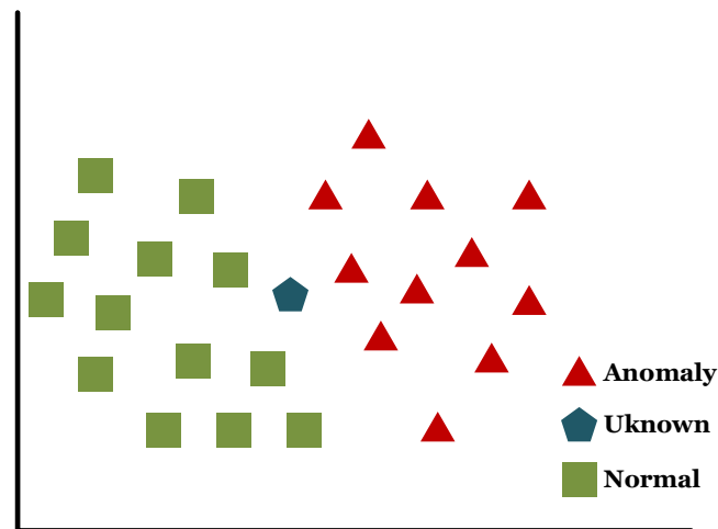
Figure 11. K-Nearest Neighbor (KNN) classification principle.
