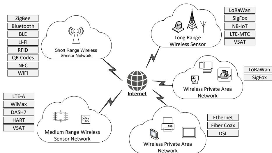
Figure 1. IoT system environment—applications and related access networks and protocols.
