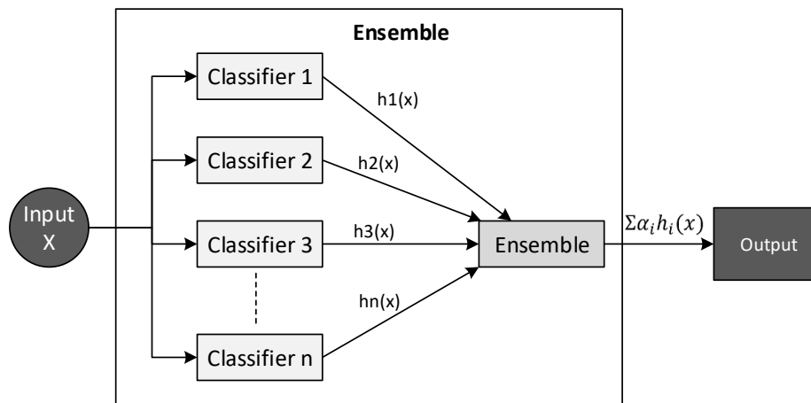
Figure 14. Working of an ensemble classifier.
