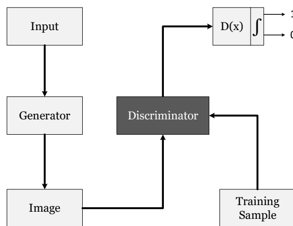
Figure 20. Illustration of generative adversarial network (GAN) working.
