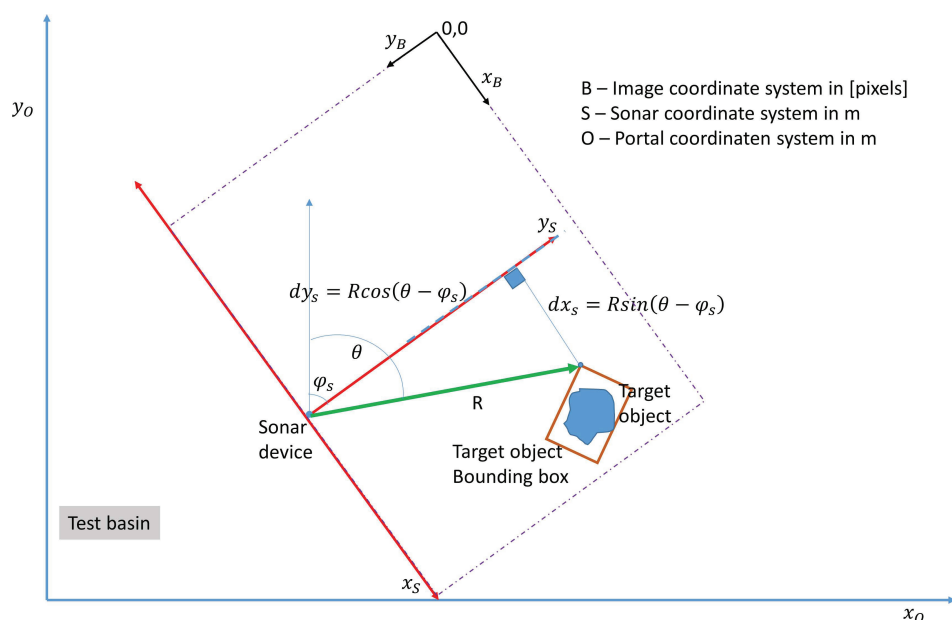
Figure 5. Geometric calculations for automatic conversion of real coordinates into sonar image coordinates for automatic image annotation.
