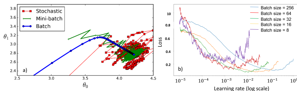
Figure 11. (a) Effects of batch sizes and (b) Relationship between learning rate error plotted using batch sizes of 8–256 for the docking station dataset.
