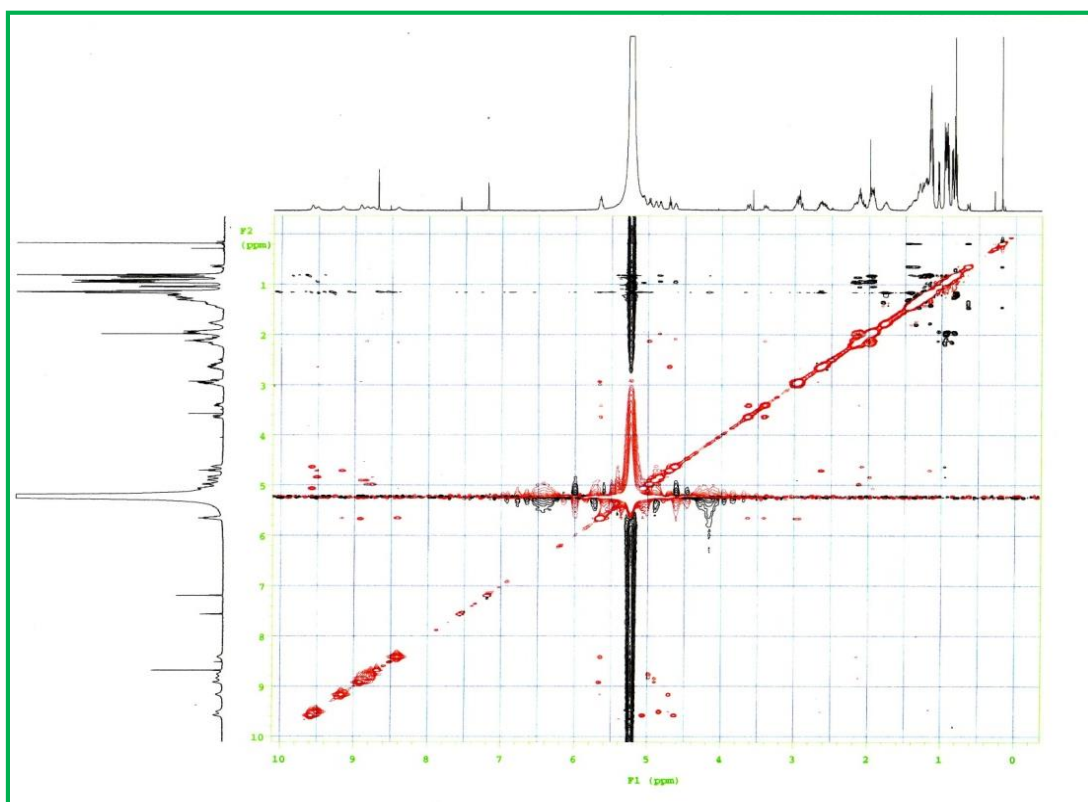
Figure S9. NOESY correlations of compound 1 (pyridine-d 5 )
