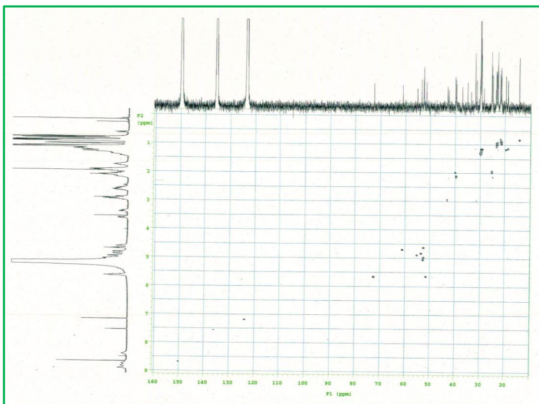
Figure S6. HSQC spectrum of compound 1 (pyridine- \text{d}_5 )
