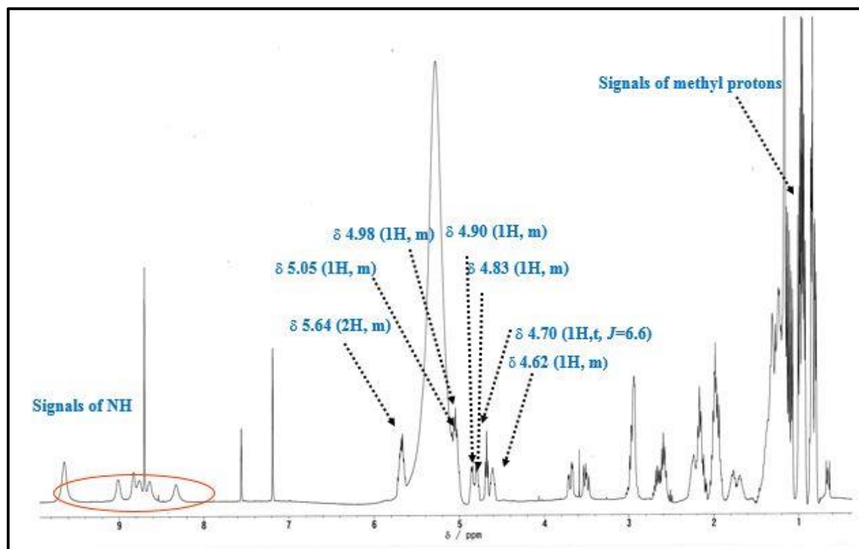
Figure S4-a. ^1\text{H-NMR} spectrum of compound 1 with identified signals
