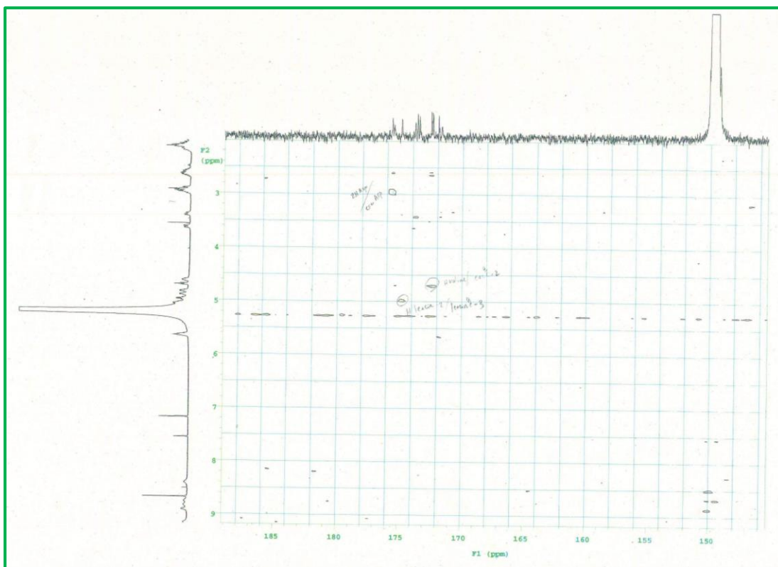
Figure S7-d. HMBC spectrum expansions of compound 1 (pyridine-d 5 )
