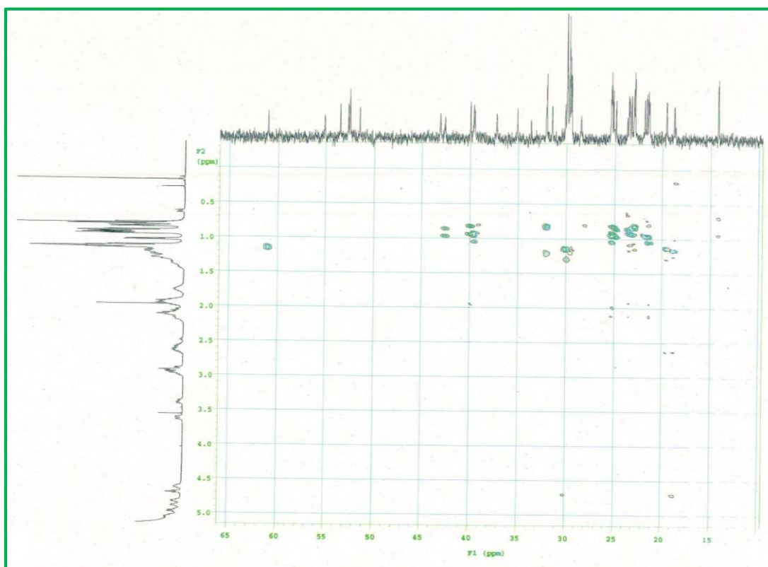
Figure S7-a. HMBC spectrum expansions of compound 1 (pyridine-d 5 )
