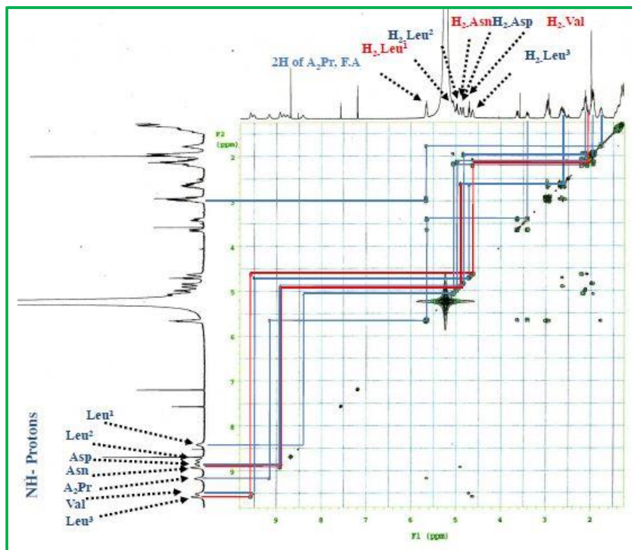
Figure S8-a. 1 H- 1 H COSY spectrum of compound 1 with identified correlations
