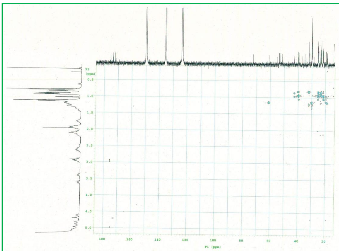
Figure S7-b. HMBC spectrum expansions of compound 1 (pyridine-d 5 )
