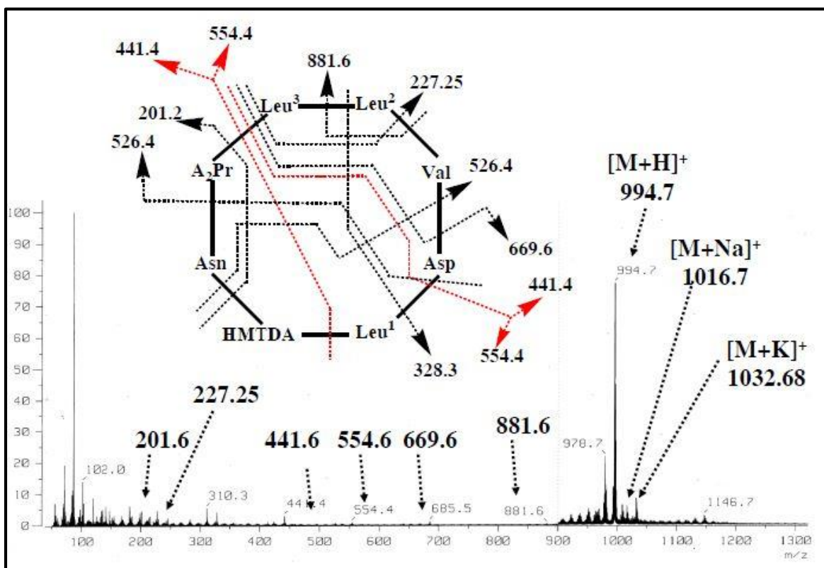
Figure S3. FABMS fragments of compound 1
