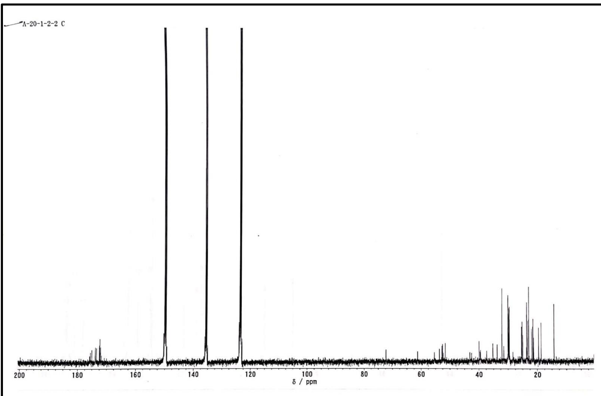
Figure S5. ^{13}\text{C} -NMR spectrum of compound 1 (pyridine- \text{d}_5 )
