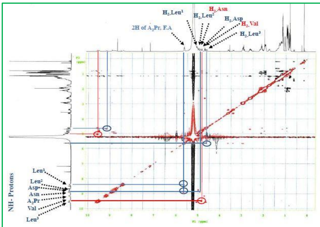
Figure S9-a. NOESY spectrum of compound 1 with identified correlations
