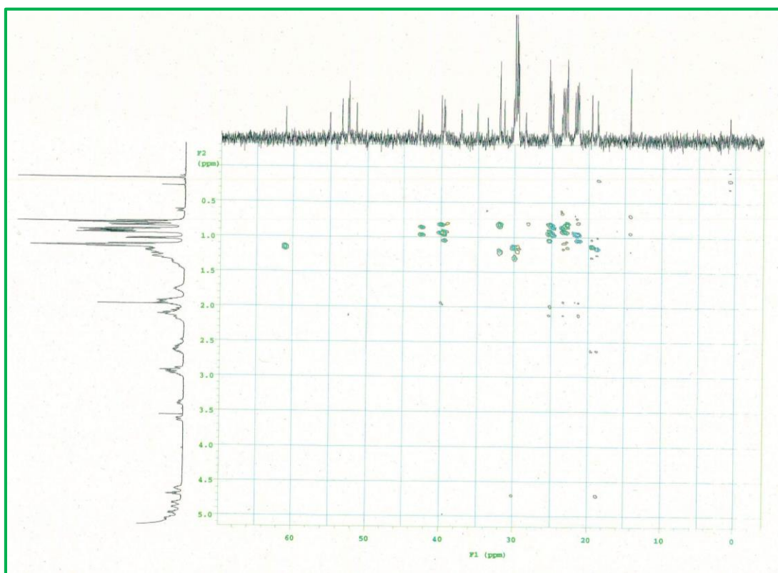
Figure S7-e. HMBC spectrum expansions of compound 1 (pyridine-d 5 )
