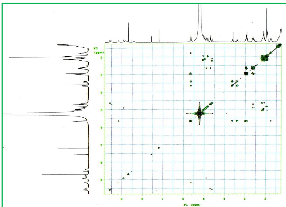
Figure S8. 1 H- 1 H COSY correlations of compound 1 (pyridine-d 5 )
