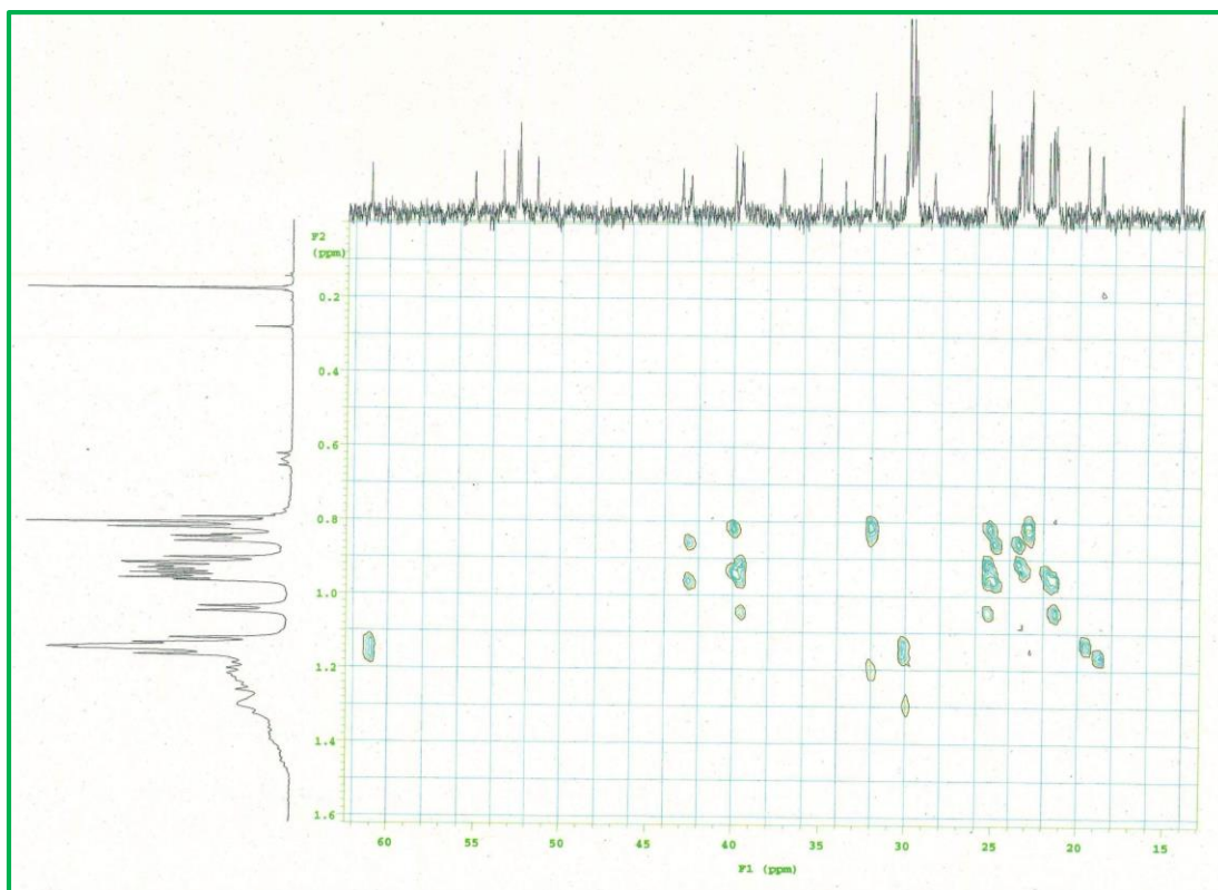
Figure S7-f. HMBC spectrum expansions of compound 1 (pyridine-d 5 )
