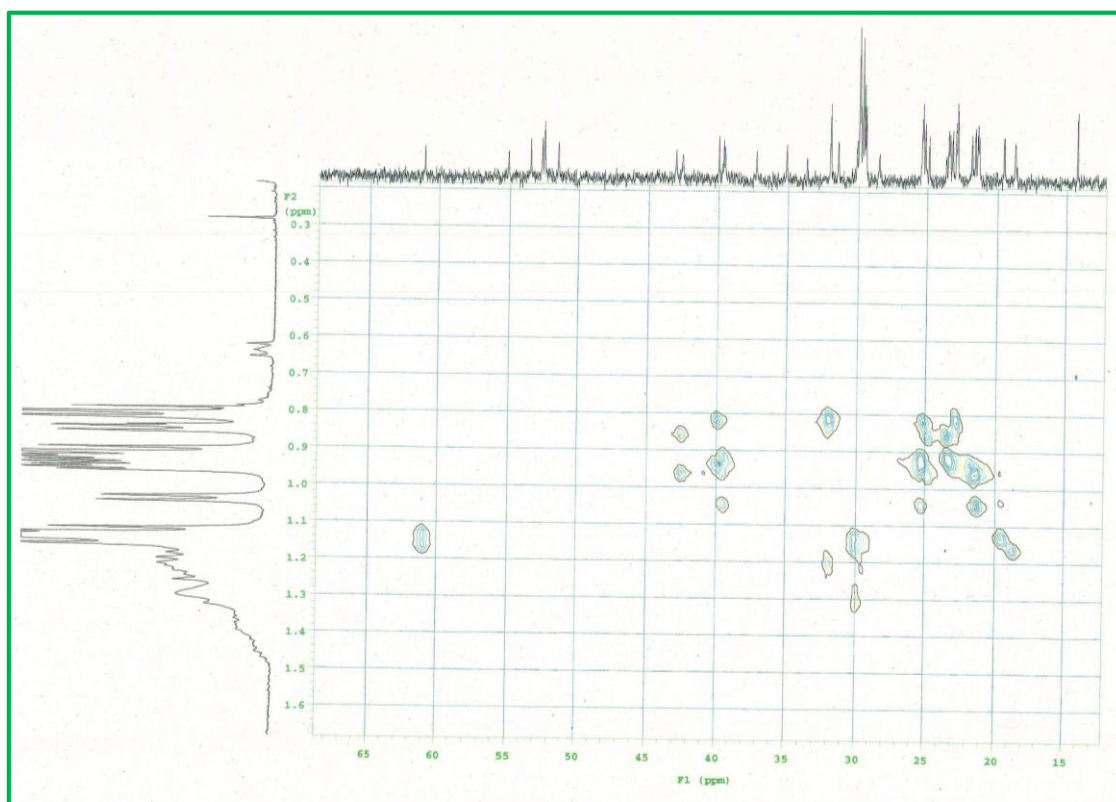
Figure S7-c. HMBC spectrum expansions of compound 1 (pyridine-d 5 )
