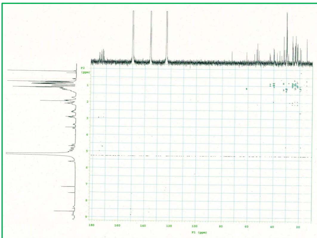
Figure S7. HMBC spectrum of compound 1 (pyridine-d 5 )
