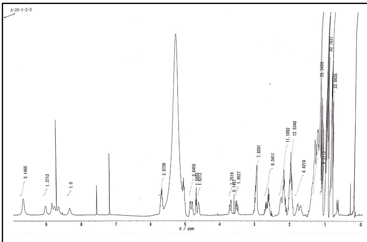
Figure S4. ^1\text{H-NMR} spectrum of compound 1 (pyridine- \text{d}_5 )
