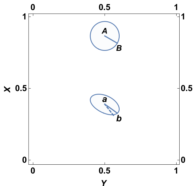
Figure 3. The galaxy cluster shape ( R_c = 0.04 ) in the plane \phi = 0 ( z = 0 ) and the line on which the rotation velocity is evaluated in inertial ( g = 0 , top ) and accelerated ( g = 0.6 , bottom ) frames for \Theta_0 = \pi/6 (‘Northern’ hemisphere). In the inertial frame, the line ( AB ) is normal to the line of sight of the cluster center. Its image ( ab ) in the accelerated frame is not normal to the line of sight of the cluster center. The normal line is shown as a dashed line.
