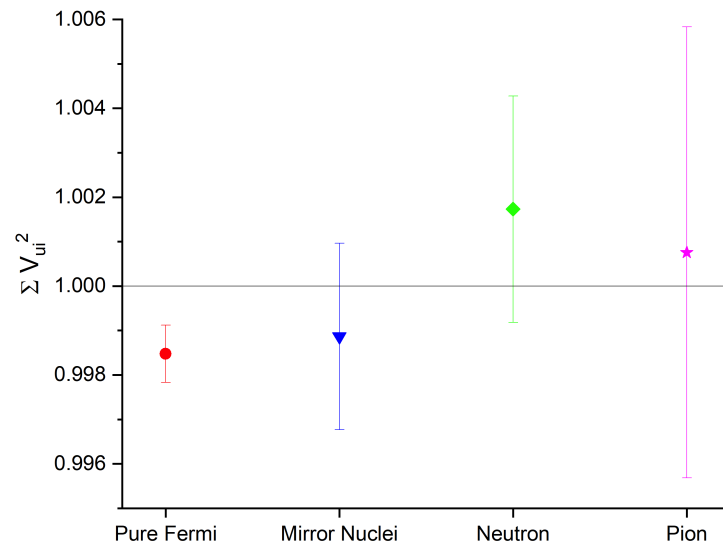
Figure 1. The current status of unitarity of the up-quark matrix mixing elements, using V_{ud} determination from pure Fermi, mixed mirror, neutron, and pion decays. The neutron decay value presented is the global average as reported in [13].
