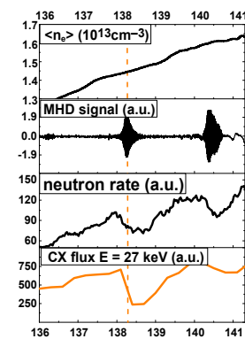
Figure 15. Correlation of neutron rate and CX flux with TAE bursts in discharge #31996. From top to bottom: line-averaged electron density, MHD signal, neutron rate, 27 keV atomic flux. The figure is taken from [45] and reproduced with permission from IOP Publishing.
