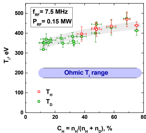
Figure 6. Ion temperature as a function of the H minority concentration in ICRH experiments (discharges ##13773–13801 with different n_H/n_D ratio). Here, T_H and T_D are the temperatures of hydrogen and deuterium ions in an ICRH experiment, and wide blue line is the ion temperature in the Ohmic regime. The figure is taken from [41] and reproduced with permission from Springer Nature.
