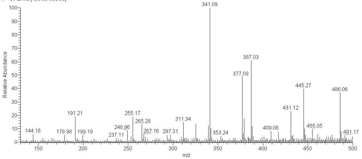
Figure S1. Electrospray ionisation–mass spectrometry (ESI-MS) spectrum of Machaerium hirtum twig extract.
