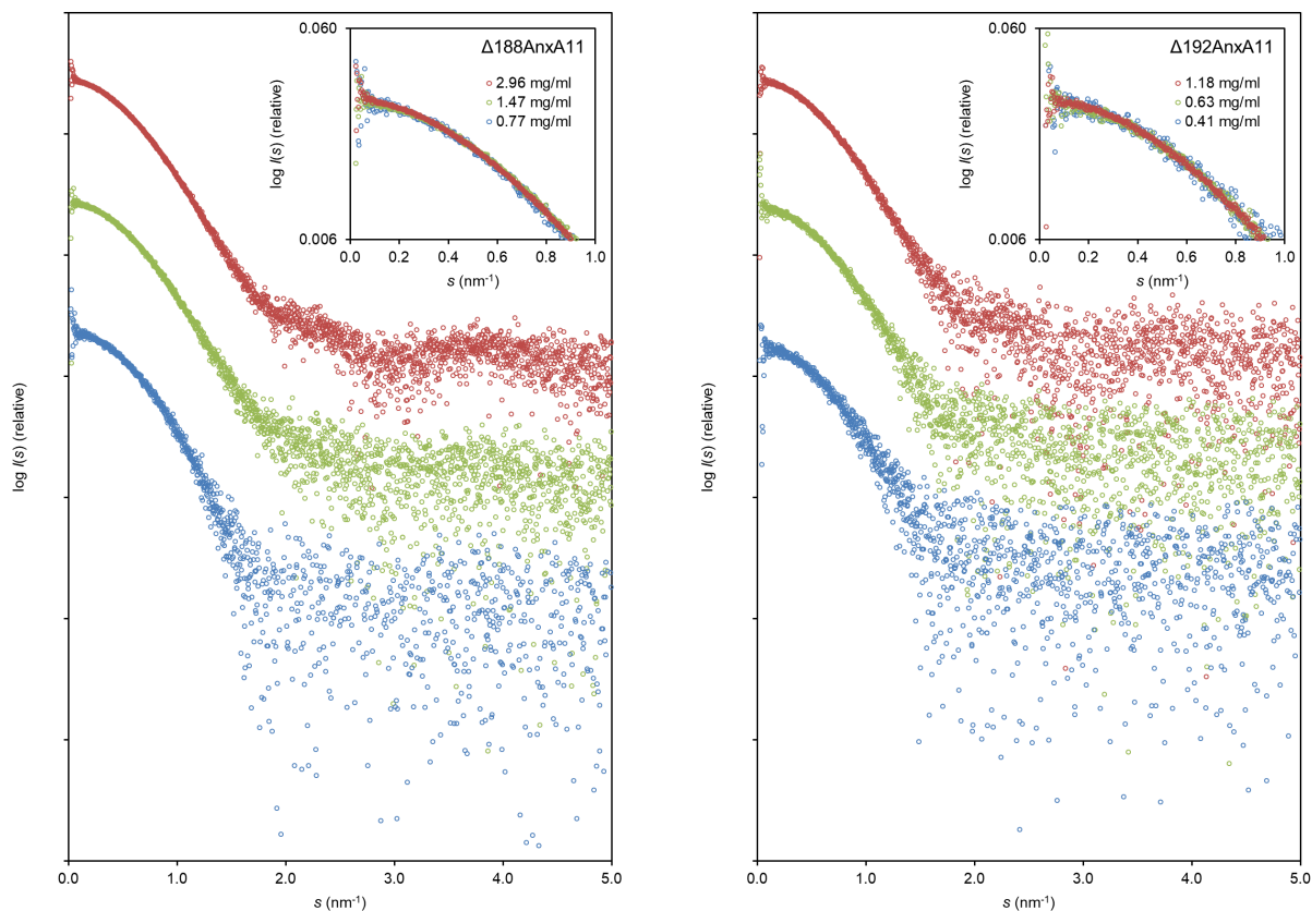
Figure S1. \Delta 188\text{AnxA11} and \Delta 192\text{AnxA11} SAXS dilution data. Background-subtracted and concentration-normalised scattering data of \Delta 188\text{AnxA11} (left) and \Delta 192\text{AnxA11} (right) are shown. The curves have been offset for clarity. The inset in both graphs shows the different concentrations superposed with one another at low angles, as well as the concentration of each dataset.
