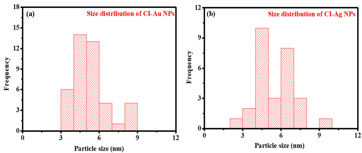
Figure S1. The particle size distribution histogram of green synthesized (a) CI-Au and (b) CI Ag NPs from TEM.
