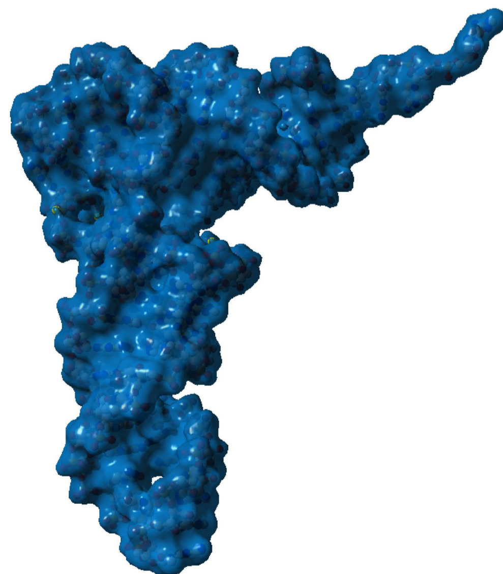
Correctly folded tRNA; Structure and function
