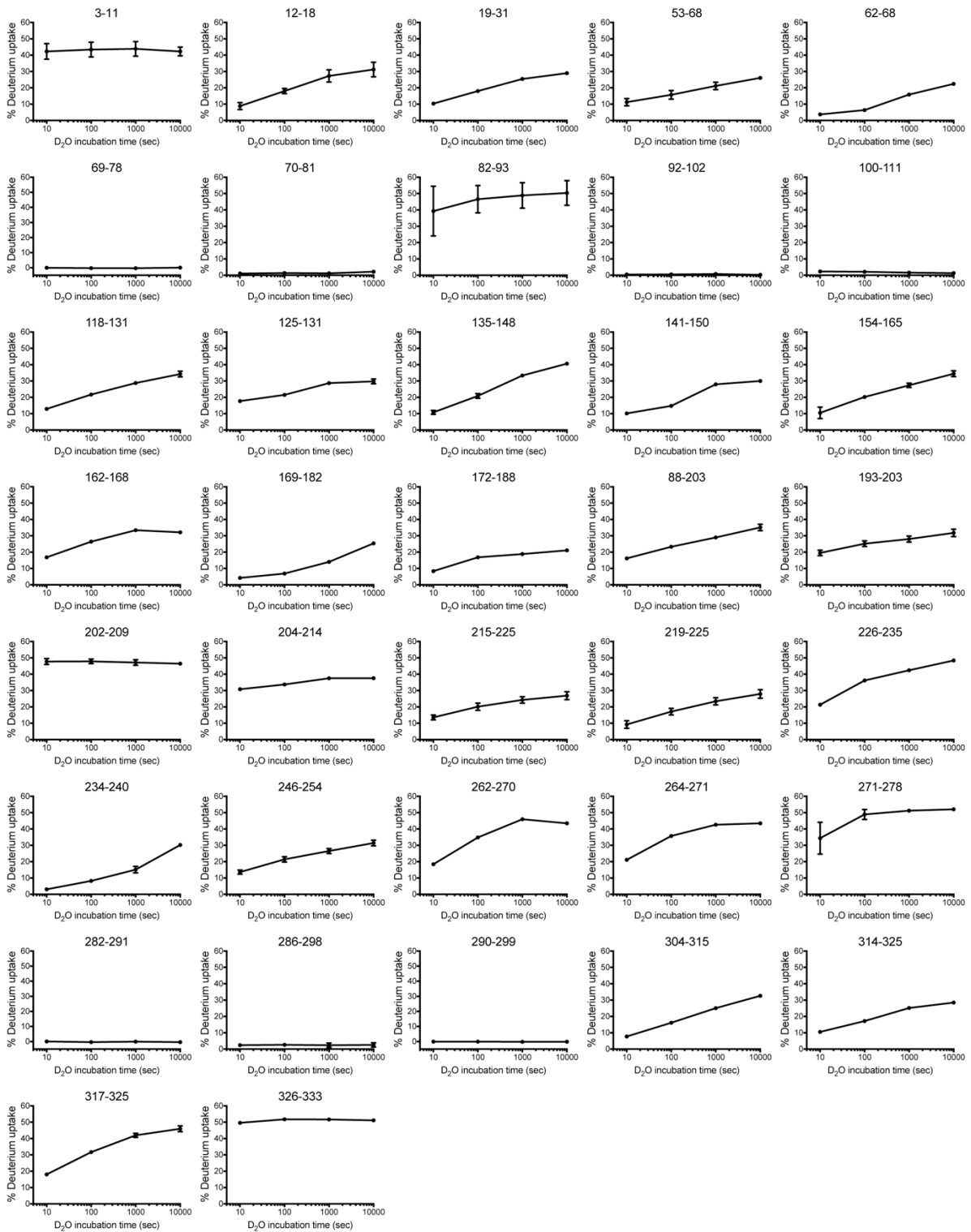
Figure S2. HDX-MS analysis of human DHDDS. Deuterium uptake plots.
