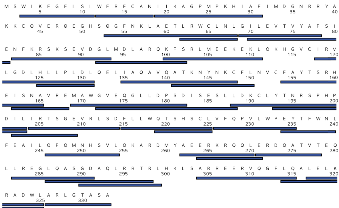
22 Figure S1. HDX-MS analysis of human DHDDS. Sequence coverage of human DHDDS.
