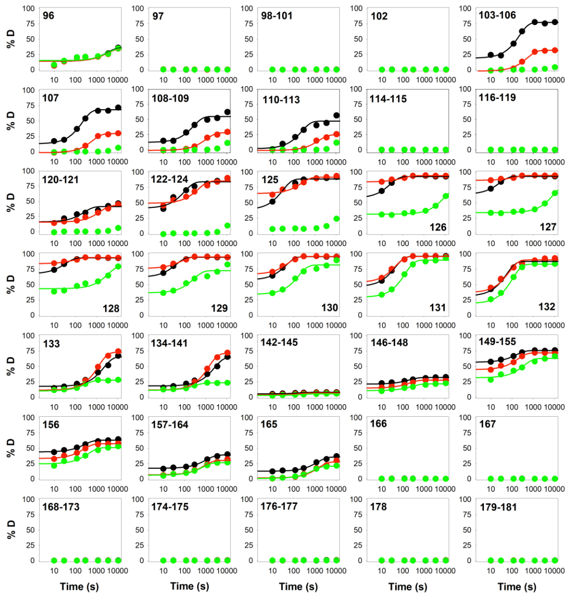
Figure S6 (2 of 3). HDX kinetics for NQO1 segments (spanning residues 96-181) of NQO1 upon FAD and dicoumarol binding. Plots show percentage of deuteration as a function of time. Segment limits are shown in each graph. Kinetic analysis can be found in Table S1.
